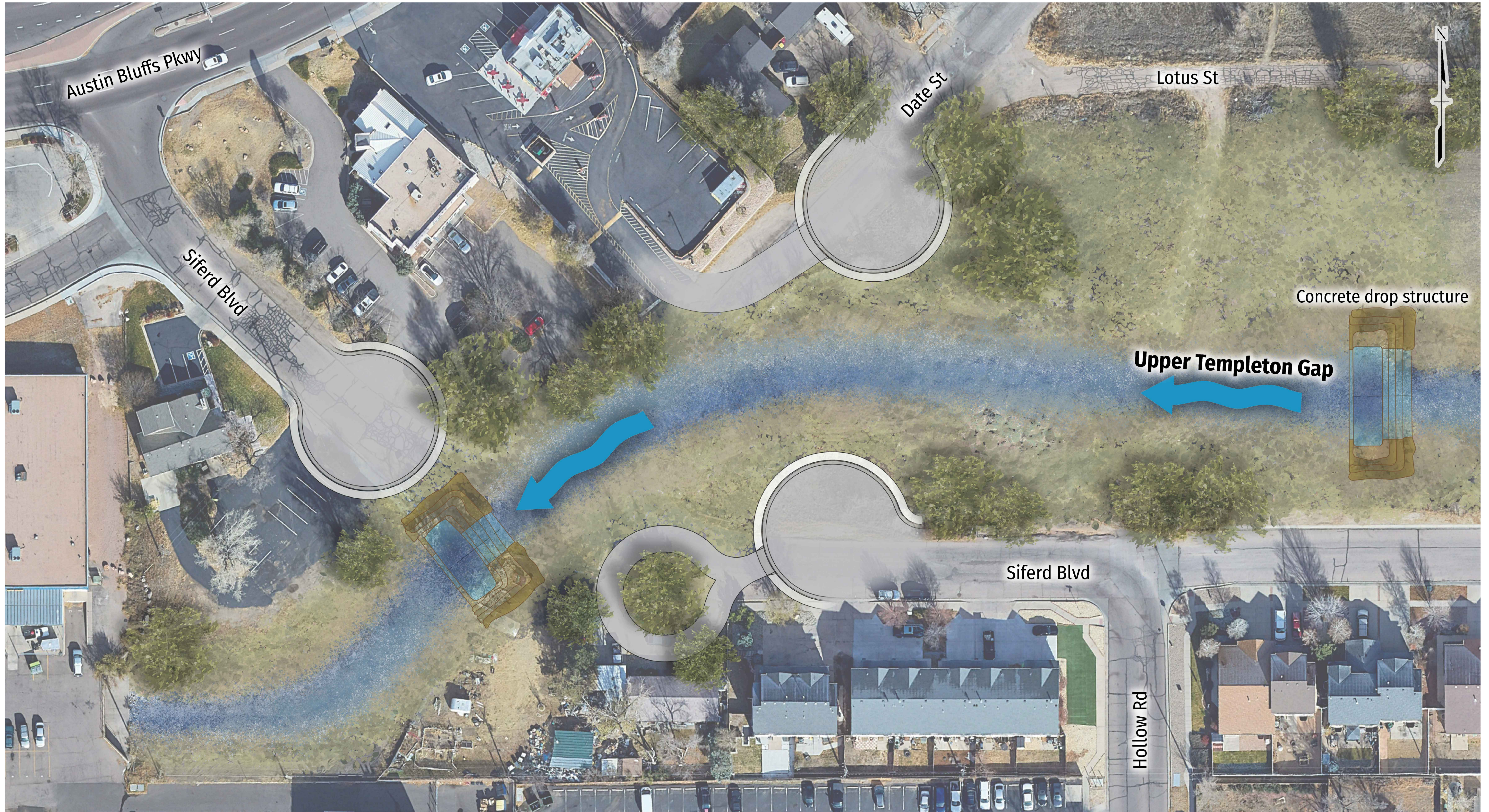
PARK VISTA CHANNEL RESTORATION PROJECT - ARTISTIC RENDERING SIFERD BLVD. AND DATE ST. - CUL-DE-SAC LOCATIONS OCTOBER 2023
